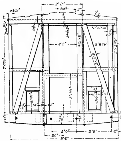
Fig. 265. End Elevation of Framing.
